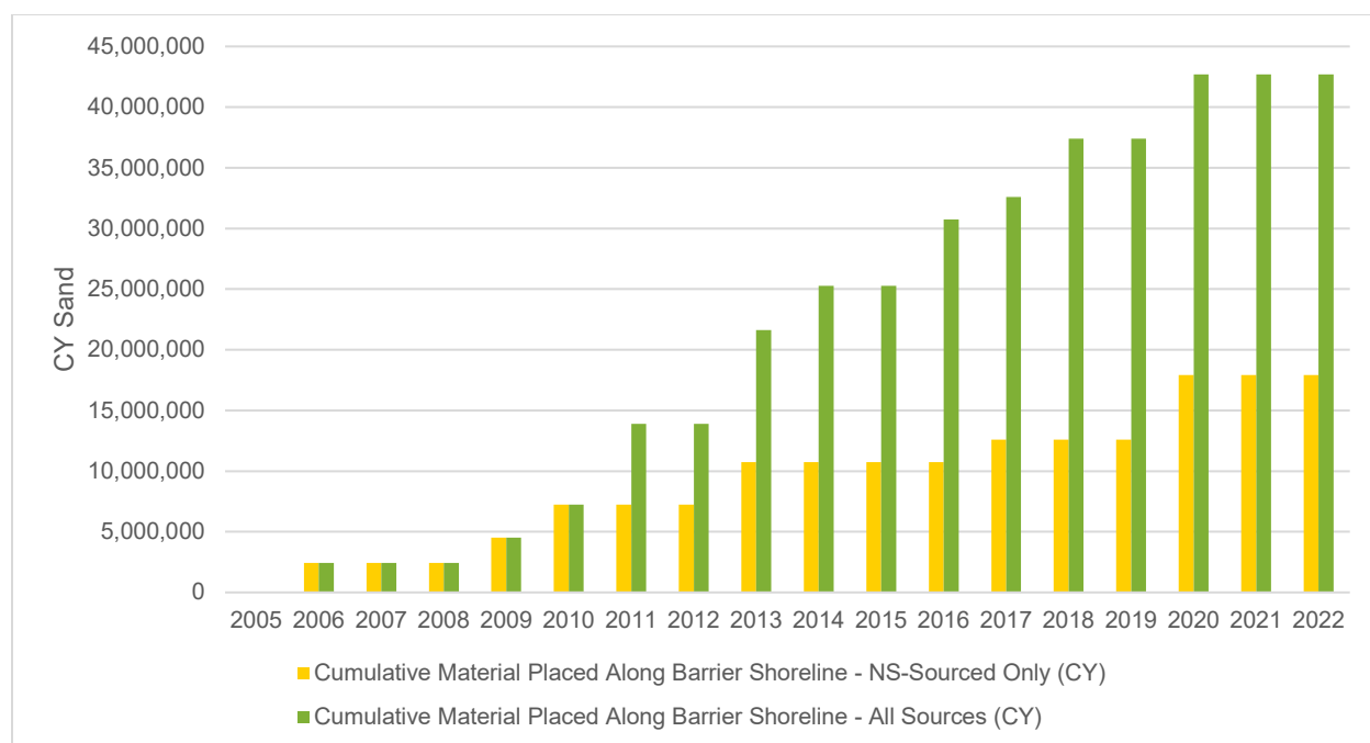
Figure 10. Amount of sand placed along the Barataria Bight shoreline from 2005 to 2022 from nearshore (NS) and all other (e.g., Ship Shoal, Mississippi River) sources.
