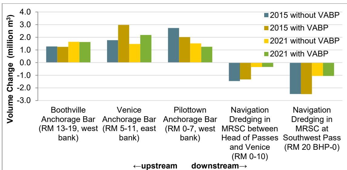
Figure 8. Volume changes at sand bars and dredged volumes from the MRSC between Venice (RM 13) and SWP (RM 20 BHP) for scenarios without and with the Venice Anchorage Borrow Pit (VABP, RM 8) for 2015 and 2021 hydrographs. From Georgiou et al. (2023).
