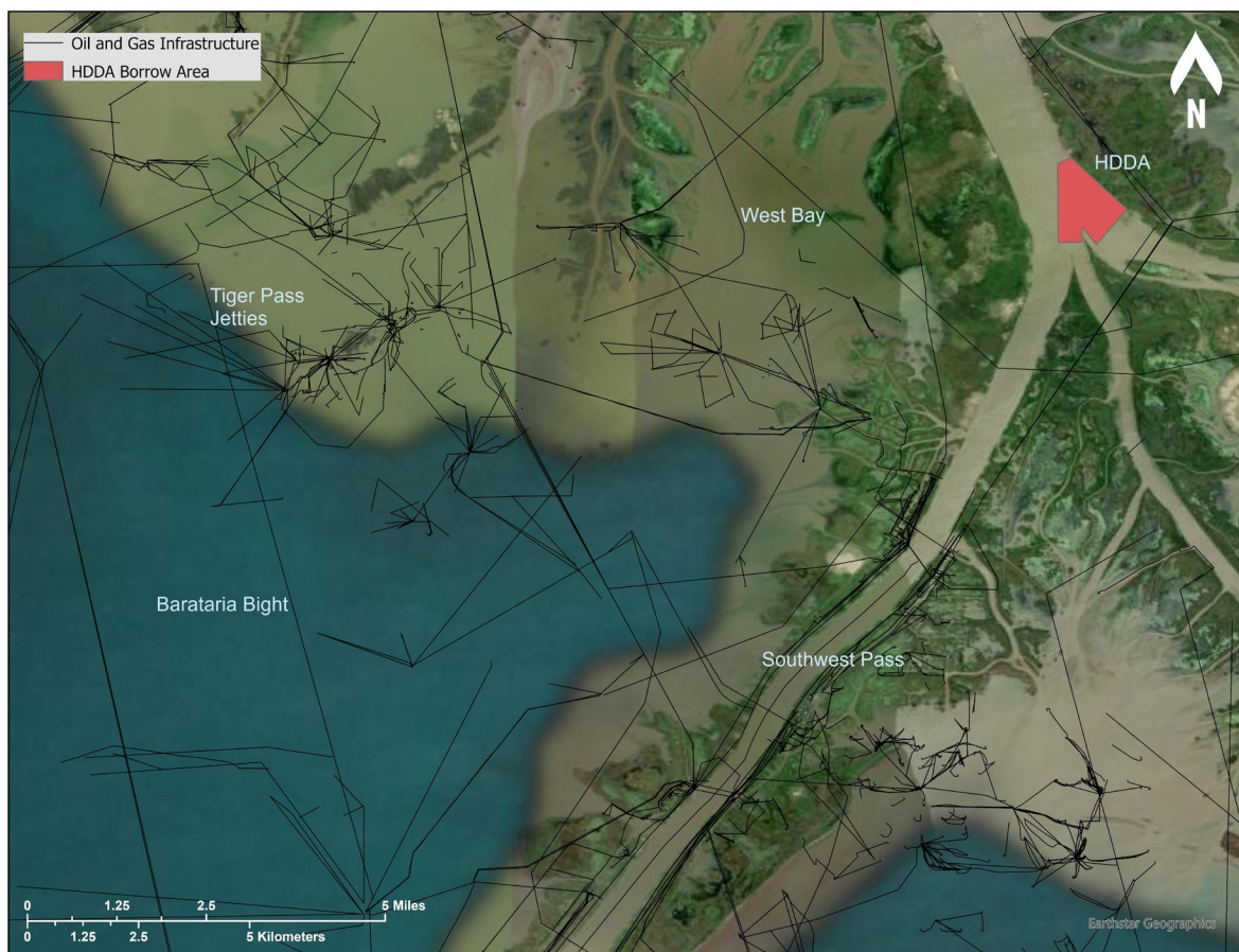
Figure 14. Location of oil and gas pipeline infrastructure in the vicinity of West Bay, LA.
