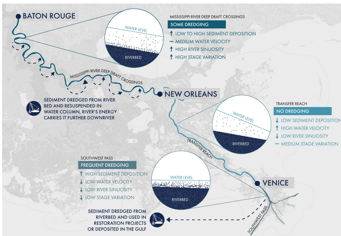
Figure 2. Sediment management reaches of the Lowermost Mississippi River.
