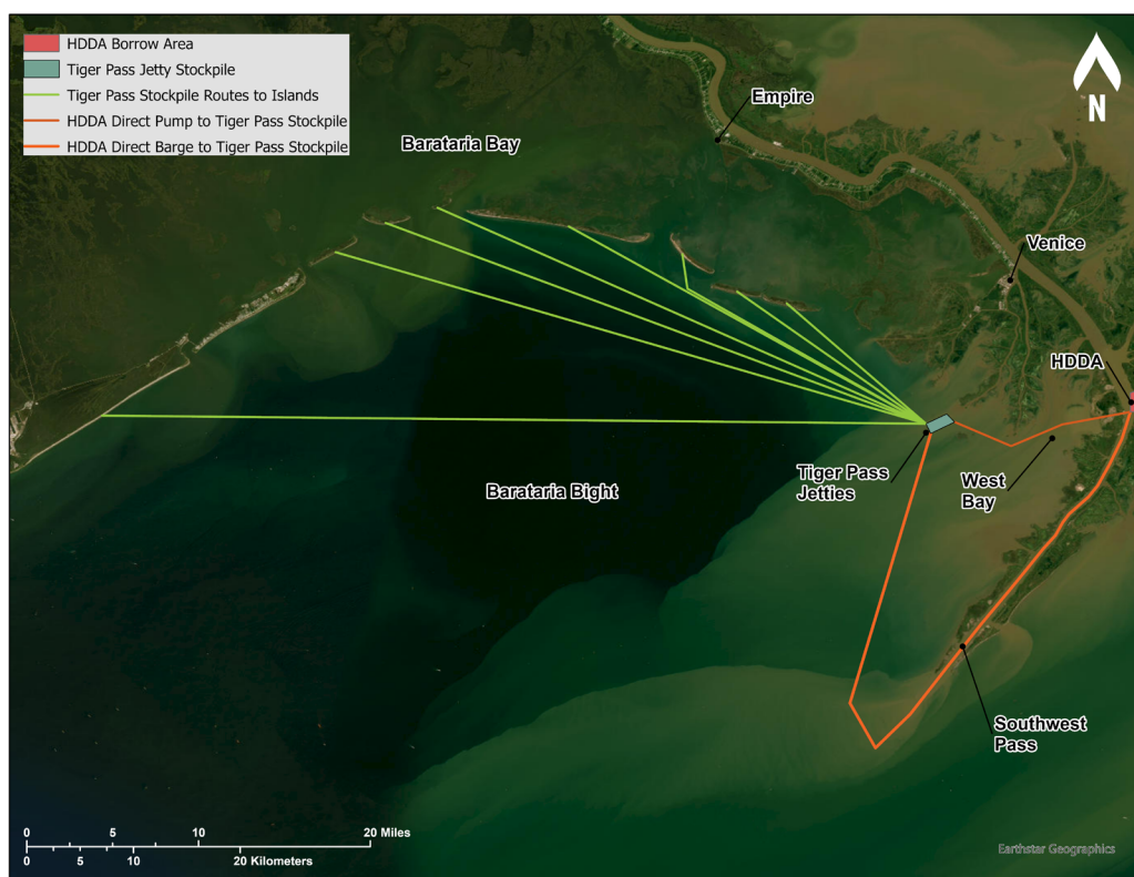
Figure 11. Tiger Pass sand stockpile alternatives group.
