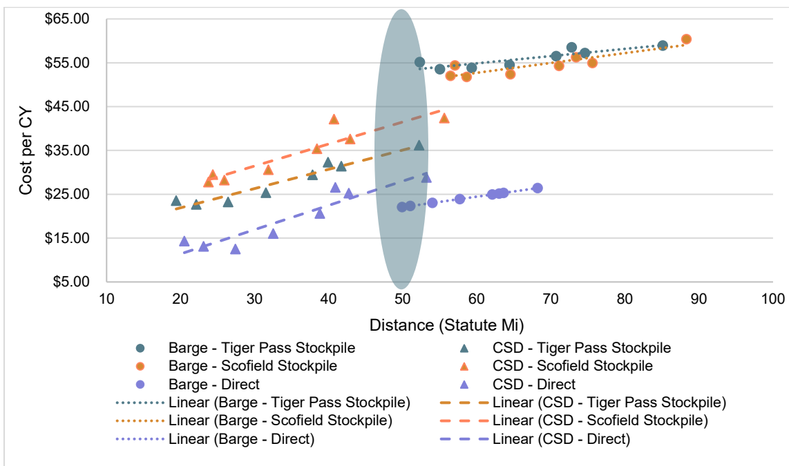
Figure 16 Total cost/CY comparison for all alternatives. Please note, these costs exclude the 50-year costs to clean out the HDDA.
