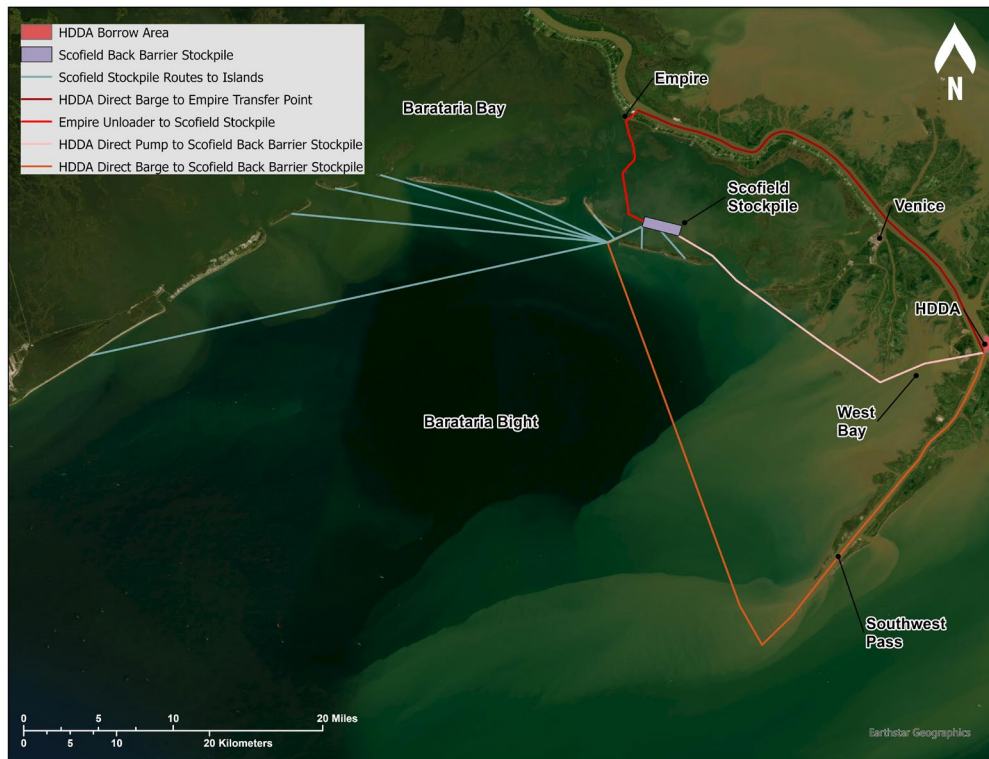
Figure 12. Scofield Island sand stockpile alternatives group.
