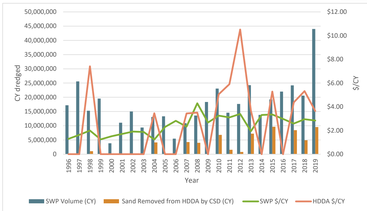
Figure 6: Comparison of total Southwest Pass dredged volumes and dredging unit costs to HDDA volumes and dredging unit costs for 1996–2019.
