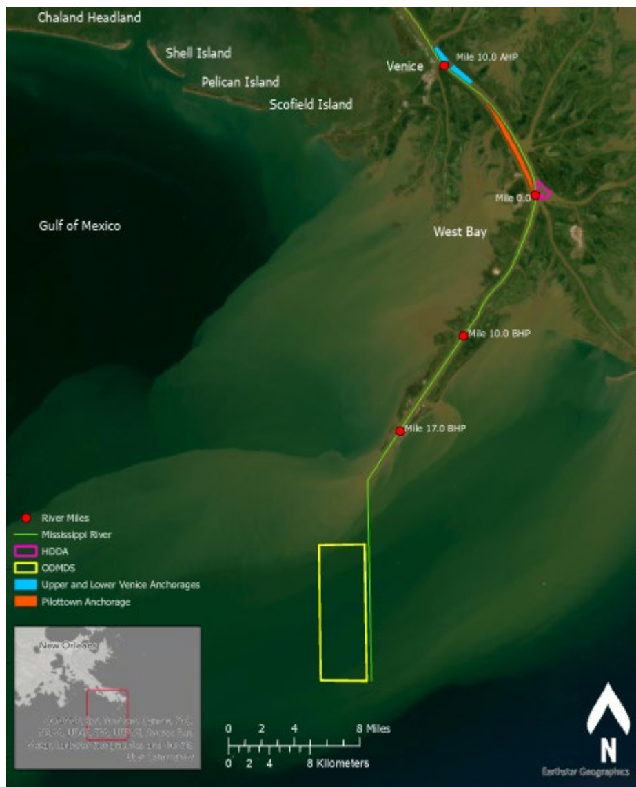
Figure 3. Lowermost Mississippi River Maintenance Dredging Regime: Material removed between RM 10.0 Above Head of Passes (AHP) and RM 11.0 BHP is placed into the HDDA for future removal or placed over bank; material removed below RM 11.0 BHP is placed over bank or into the ODMDS. Adopted from (USACE, 2018).
