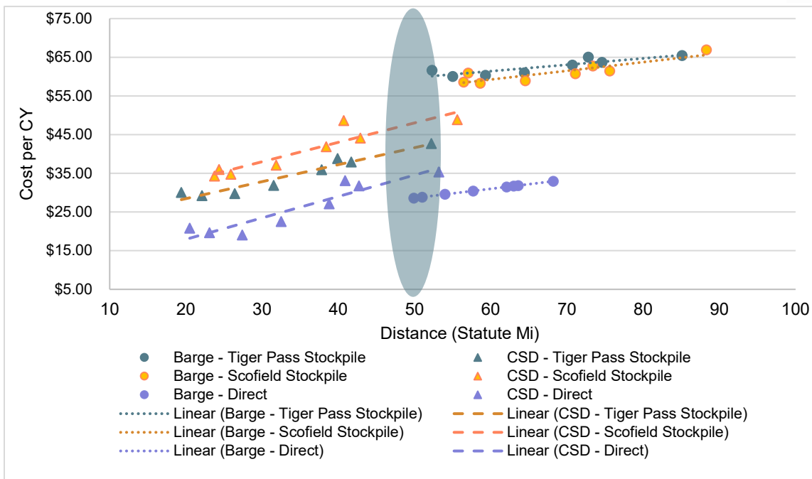
Figure 15. Total cost/CY comparison for all alternatives. Please note, these costs are inclusive of the 50-year costs to clean out the HDDA.
