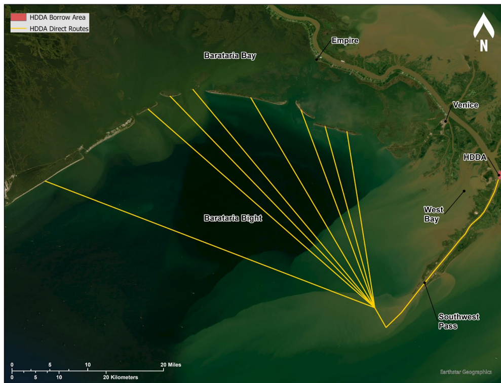
Figure 13. Direct sand transport via CSD and barge alternative.
